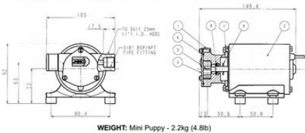
DIMENSIONAL DRAWING & PARTS LIST
