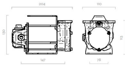
Dimensions expressed in millimeters
