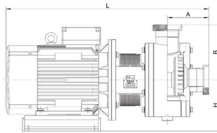
■ Dimension drawing DLM/H (KB)
