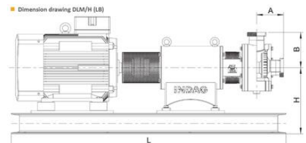
■ Dimension drawing DLM/H (LB)
