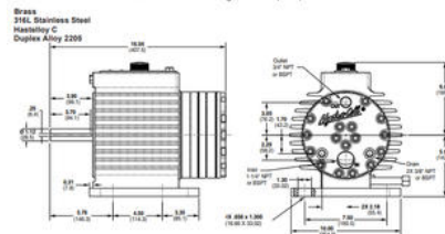
D/G17 Models for Vertical Mounting Inches (mm)
