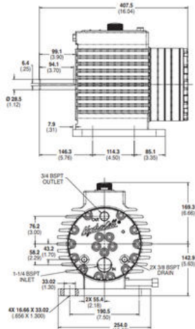
G15 Models with Metallic Pump Head mm (Inches)
