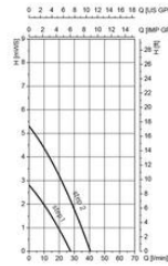
Performance charts*
