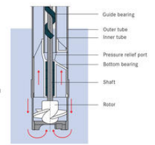
F 314, FP 314 - The small sealless drum pump
